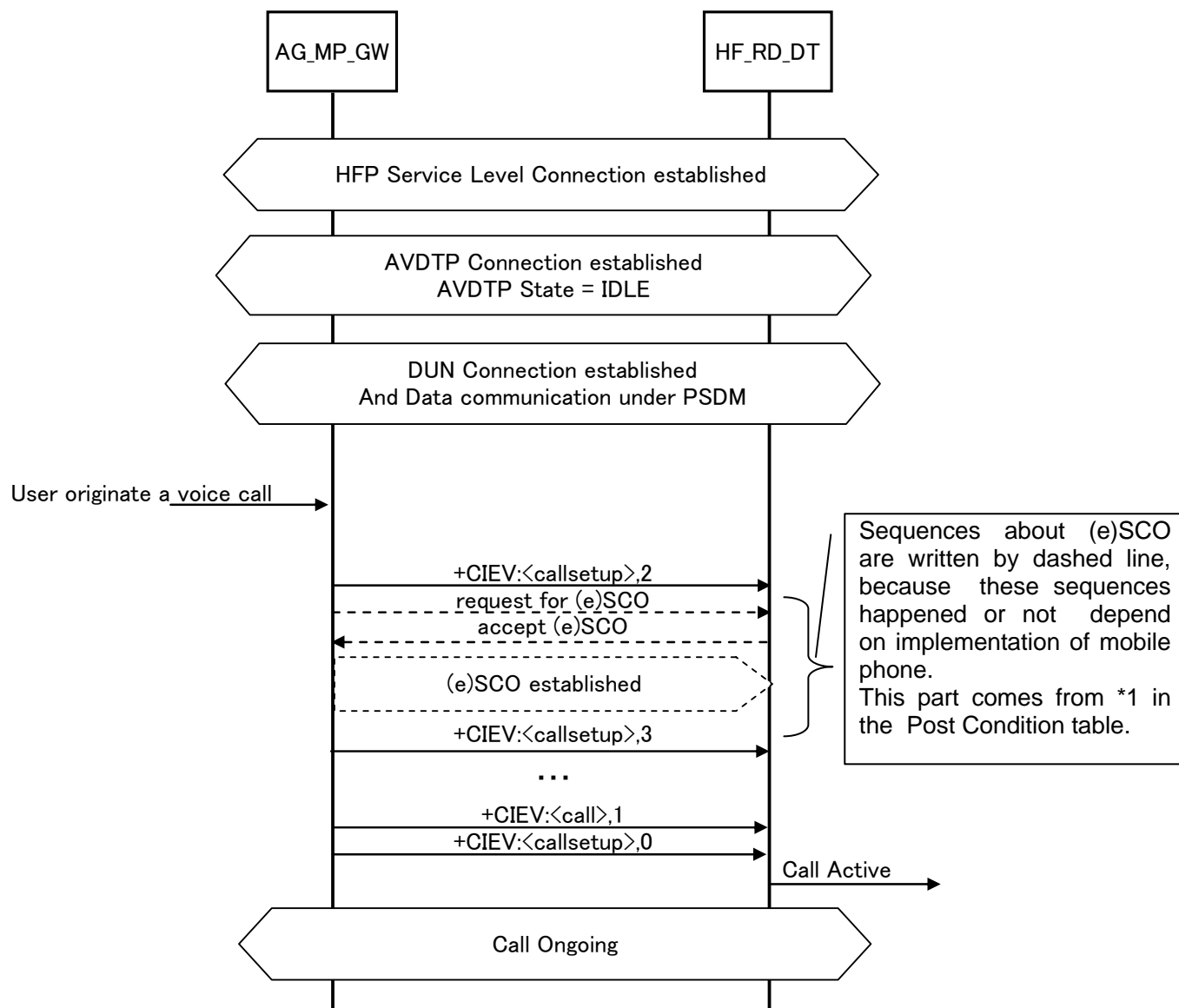
Figure 4.2.5.5. HFP+A2DP/VDP+AVRCP+DUN; OUTGOING CALL UNDER PACKET-SWITCHED DATA MODE. (User initiates a voice call on AG_MP_GW)
