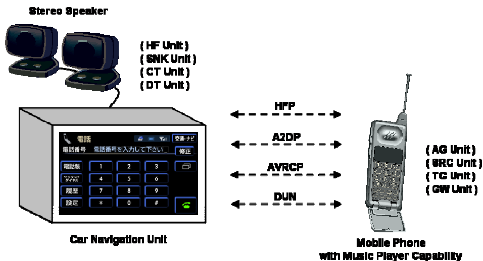
Figure 2.2 example system configuration Case 2 (Same Device Scenario)
