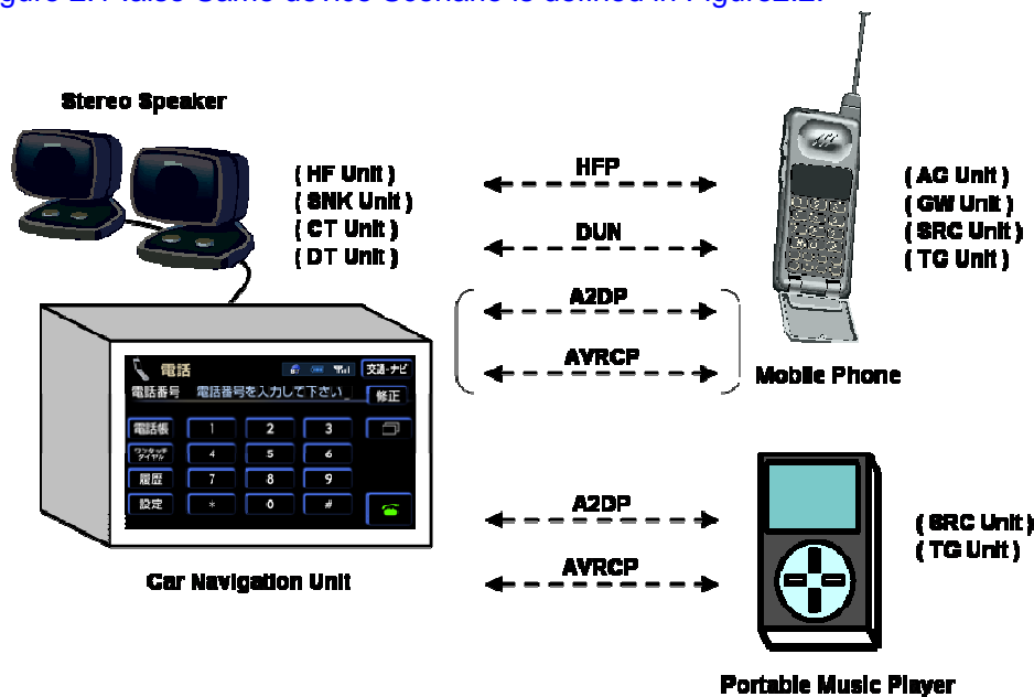
Figure 2.1 example system configuration Case 1 (Third Device Scenario)
