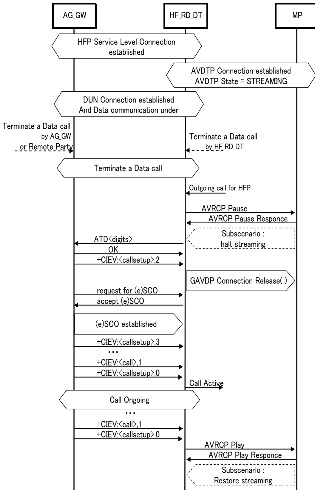
Figure 4.3.7.5. HFP+A2DP/VDP+AVRCP+DUN; OUTGOING CALL WHILE LISTENING TO MUSIC DATA COMMUNICATION UNDER CIRCUIT-SWITCHED DATA MODE IN CASE OF THE THIRD DEVICE. (HF_RD_DT initiated)
