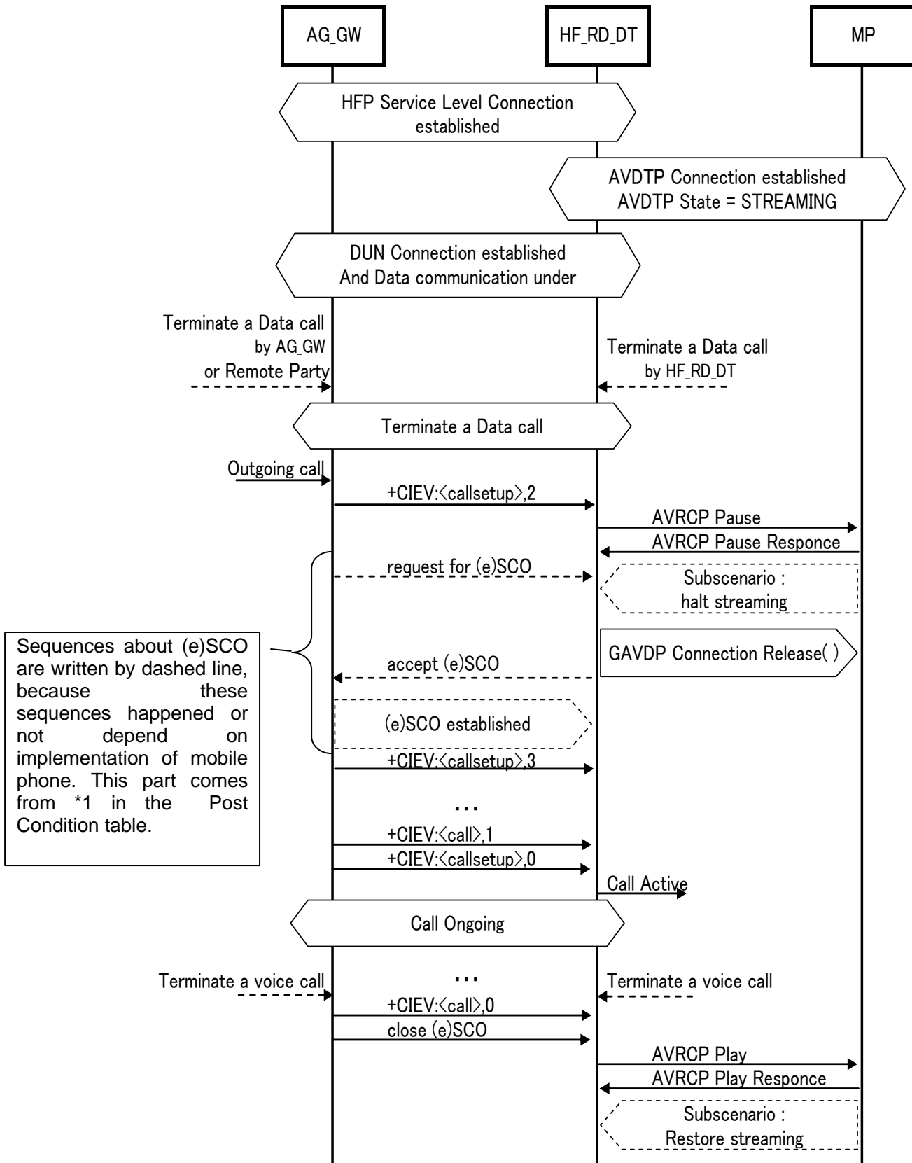
Figure 4.3.7.5. HFP+A2DP/VDP+AVRCP+DUN; OUTGOING CALL WHILE LISTENING TO MUSIC DATA COMMUNICATION UNDER CIRCUIT-SWITCHED DATA MODE IN CASE OF THE THIRD DEVICE. (AG_GW initiated)
