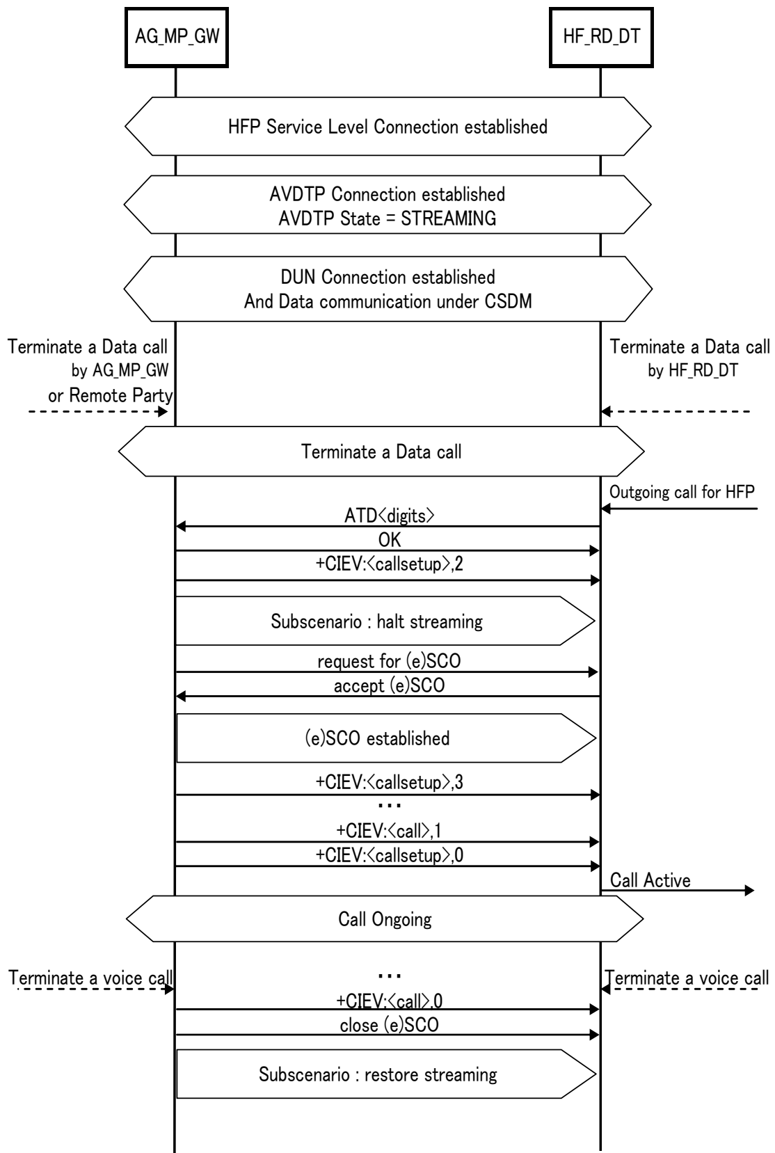
Figure 4.2.7.5. HFP+A2DP/VDP+AVRCP+DUN; OUTGOING CALL WHILE LISTENING TO MUSIC AND DATA COMMUNICATION UNDER CIRCUIT-SWITCHED DATA MODE. (HF_RD_DT initiated)
