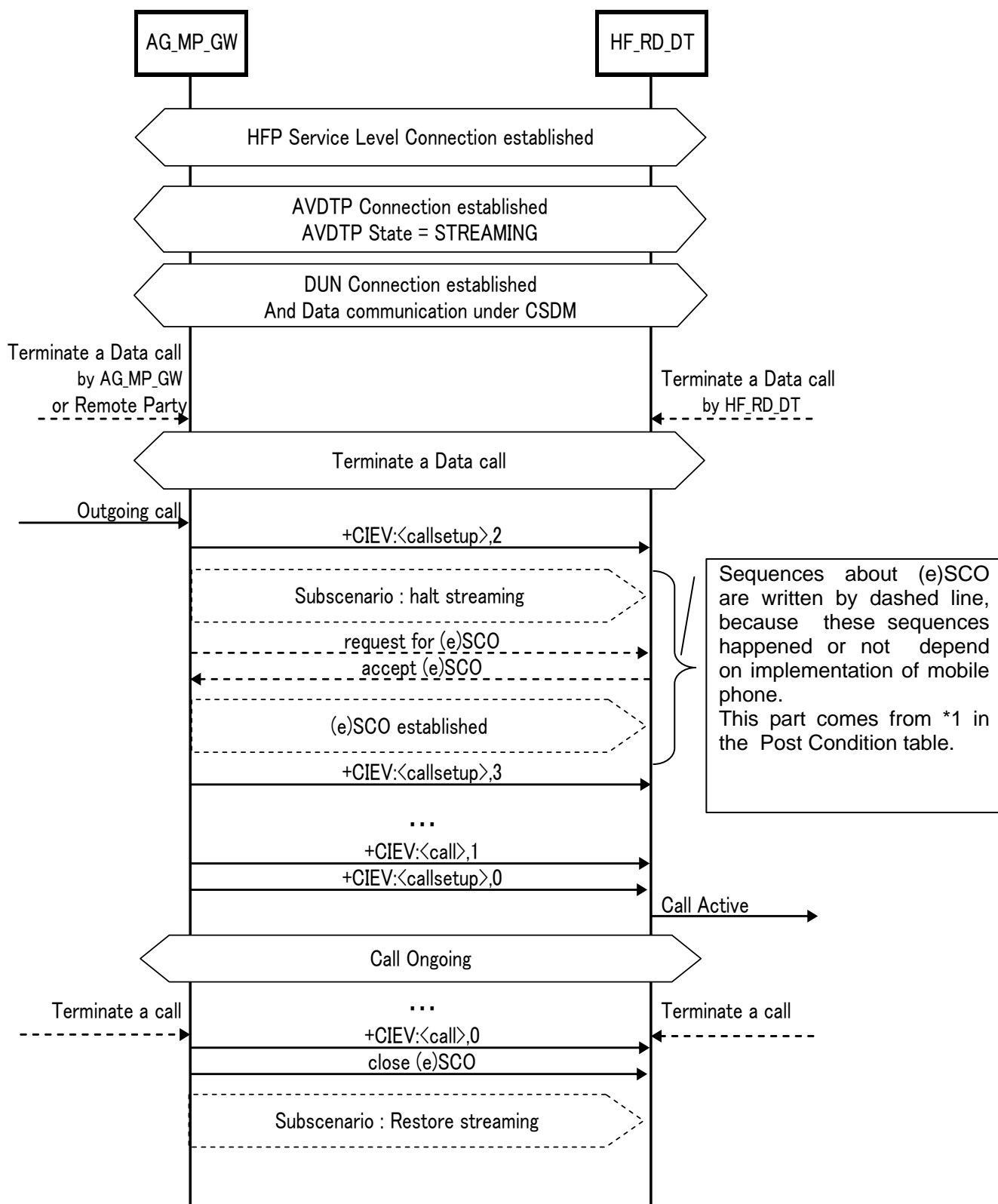
Figure 4.2.7.5. HFP+A2DP/VDP+AVRCP+DUN; OUTGOING CALL WHILE LISTENING TO MUSIC AND DATA COMMUNICATION UNDER CIRCUIT-SWITCHED DATA MODE. (AG_MP_GW initiated)
